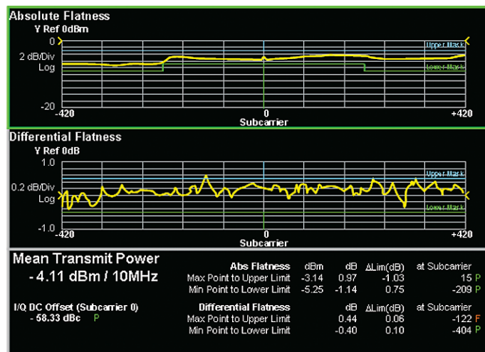
Figure 4. The standard-specific measurement application also provides graphical results paired with limit lines and pass/fail testing.
