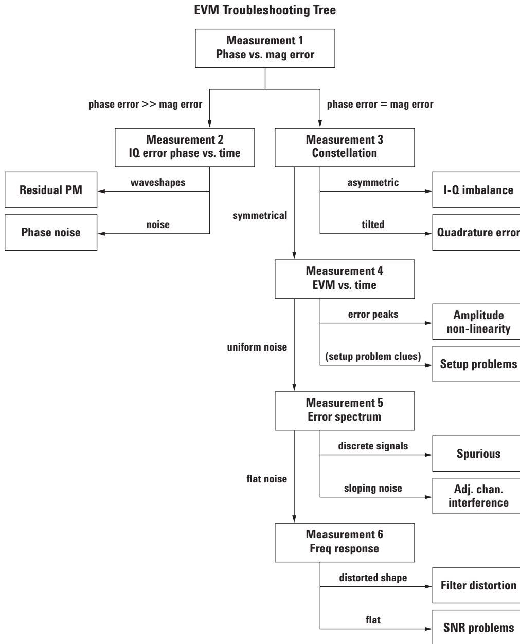
Figure 7. Error vector measurements are most effective for finding problems when used in an organized manner. This tree describes a sequence of measurements and evaluations that will focus troubleshooting efforts. More branches could be added to this tree for use on specific modulation schemes such as OFDM and CDMA.
