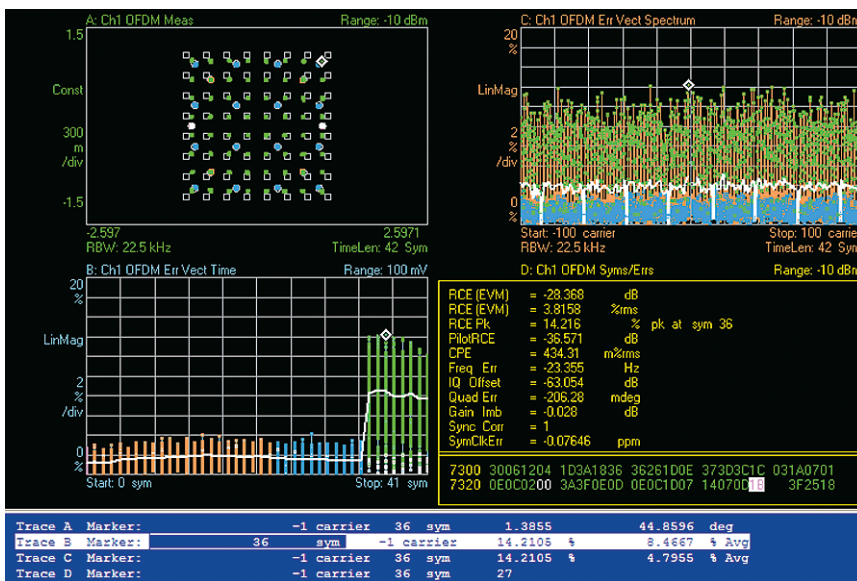
Figure 5. A basic digital demodulation result from the MXA's 89601A VSA measurement application including a constellation diagram and a composite table of error parameters and measured symbols, along with the two main error vector displays of error vs. time (lower left) and symbol and error vs. frequency (upper right). Marker coupling is used to correlate a peak in the error vector time trace across several displays and measurement domains.
