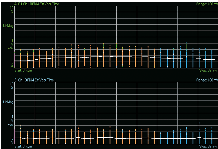
Figure 6. The magnitude portion of the error vector signal reveals the effect of pilot tracking. In the bottom trace amplitude tracking has been used, removing the amplitude drift which is evident in the top trace. Amplitude tracking improved the RCE (EVM) by about 5 dB.
