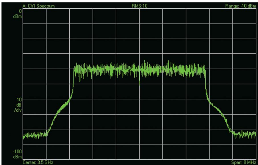
Figure 1. This basic spectrum measurement reveals much about an OFDM signal, though its untriggered averaging of a pulsed signal introduces some uncertainties. This measurement is good for determining the signal center frequency and approximate bandwidth, average power and flatness, and verifying the missing (normally untransmitted) center carrier.
